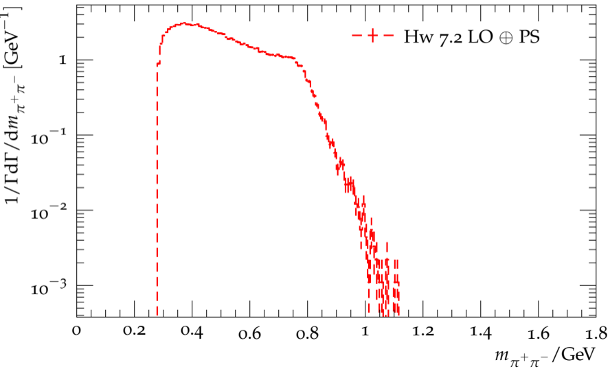
Distribution of the \pi^+\pi^- mass for \tau^- \rightarrow 3\pi^- 2\pi^+ \nu_\tau
