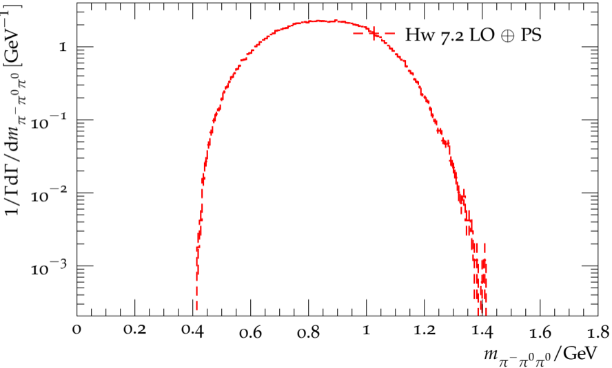
Distribution of the \pi^- \pi^0 \pi^0 mass for \tau^- \rightarrow 2\pi^0 2\pi^- \pi^+ \nu_\tau
