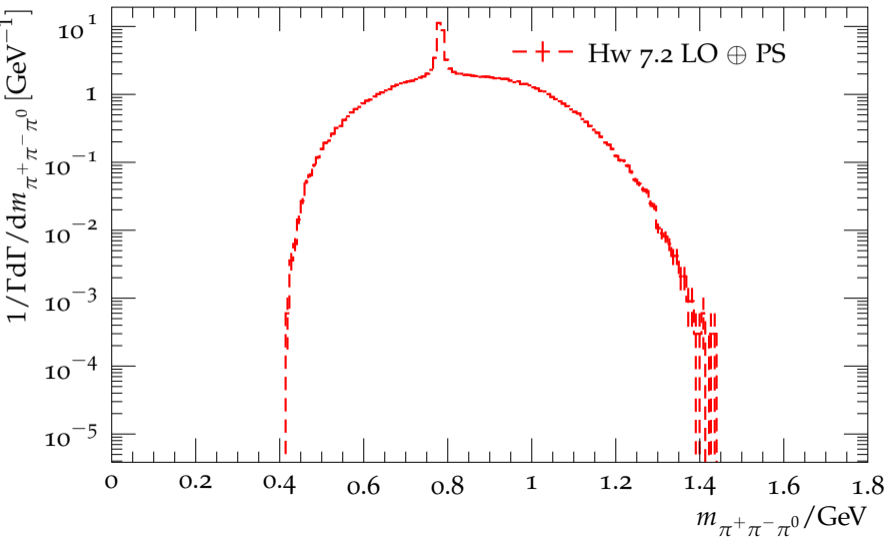
Distribution of the \pi^+\pi^-\pi^0 mass for \tau^- \rightarrow 2\pi^0 2\pi^-\pi^+ \nu_\tau
