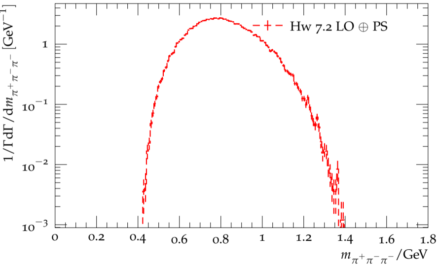
Distribution of the \pi^+\pi^-\pi^- mass for \tau^- \rightarrow 2\pi^0 2\pi^-\pi^+\nu_\tau
