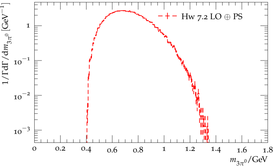
Distribution of the 3\pi^0 mass for \tau^- \rightarrow 4\pi^0\pi^-\nu_\tau
