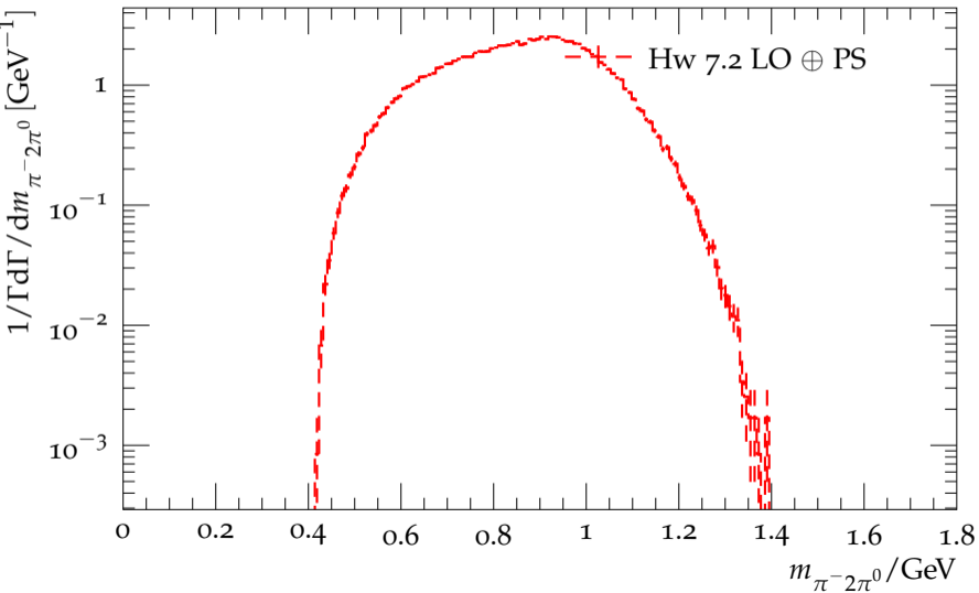
Distribution of the \pi^- 2\pi^0 mass for \tau^- \rightarrow 4\pi^0 \pi^- \nu_\tau
