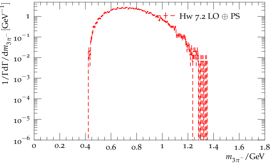
Distribution of the 3\pi^- mass for \tau^- \rightarrow 3\pi^- 2\pi^+ \nu_\tau
