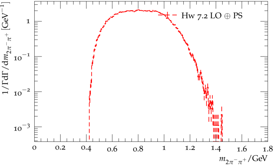
Distribution of the 2\pi^- \pi^+ mass for \tau^- \rightarrow 3\pi^- 2\pi^+ \nu_\tau
