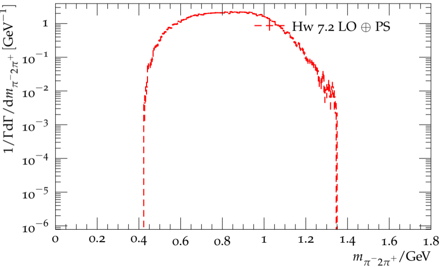
Distribution of the \pi^-2\pi^+ mass for \tau^- \rightarrow 3\pi^-2\pi^+\nu_\tau
