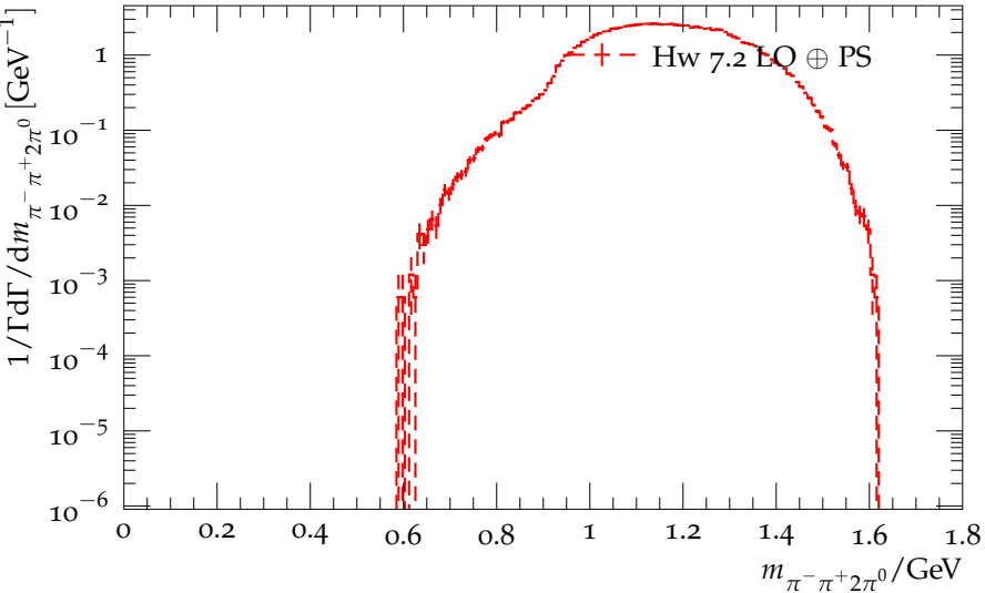
Distribution of the \pi^- \pi^+ 2\pi^0 mass for \tau^- \rightarrow 2\pi^0 2\pi^- \pi^+ \nu_\tau
