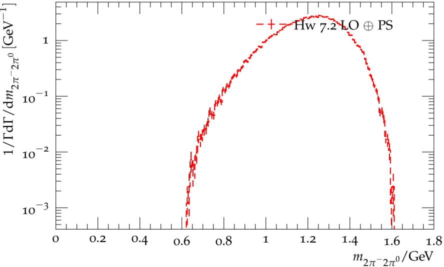
Distribution of the 2\pi^-2\pi^0 mass for \tau^- \rightarrow 2\pi^0 2\pi^- \pi^+ \nu_\tau
