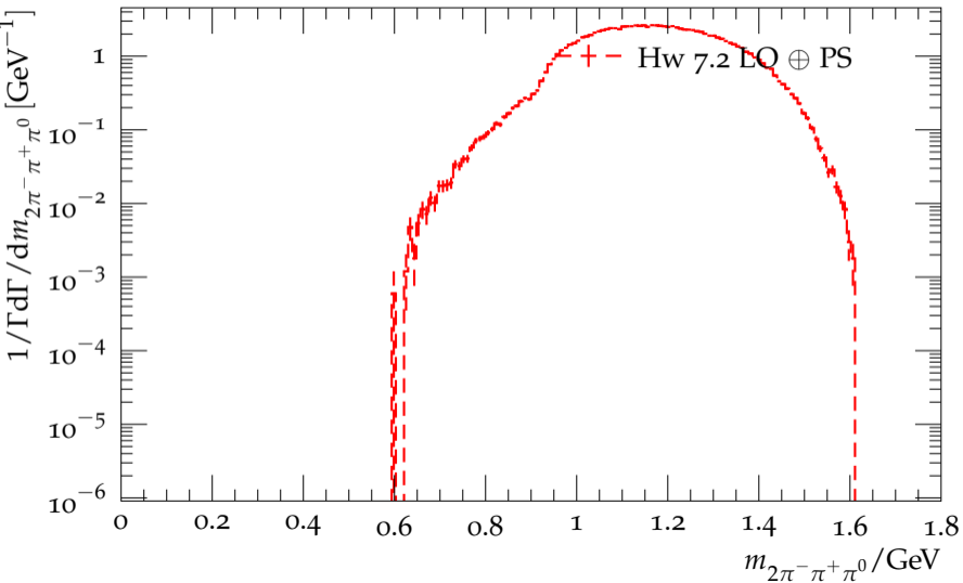
Distribution of the 2\pi^-\pi^+\pi^0 mass for \tau^- \rightarrow 2\pi^0 2\pi^-\pi^+\nu_\tau
