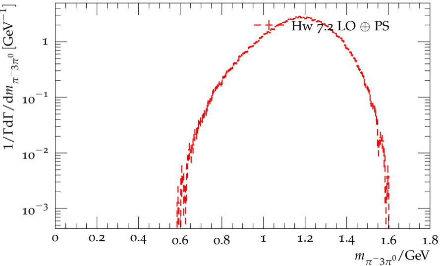
Distribution of the \pi^- 3\pi^0 mass for \tau^- \rightarrow 4\pi^0 \pi^- \nu_\tau
