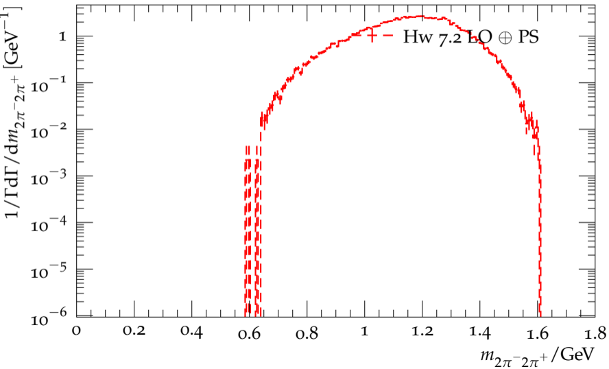
Distribution of the 2\pi^-2\pi^+ mass for \tau^- \rightarrow 3\pi^-2\pi^+\nu_\tau
