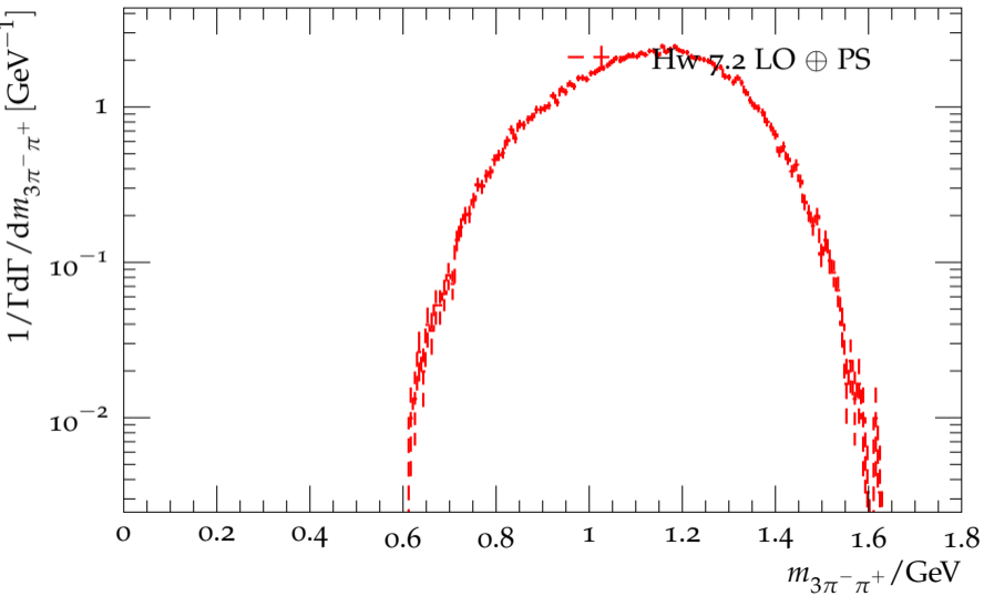
Distribution of the 3\pi^-\pi^+ mass for \tau^- \rightarrow 3\pi^- 2\pi^+ \nu_\tau
