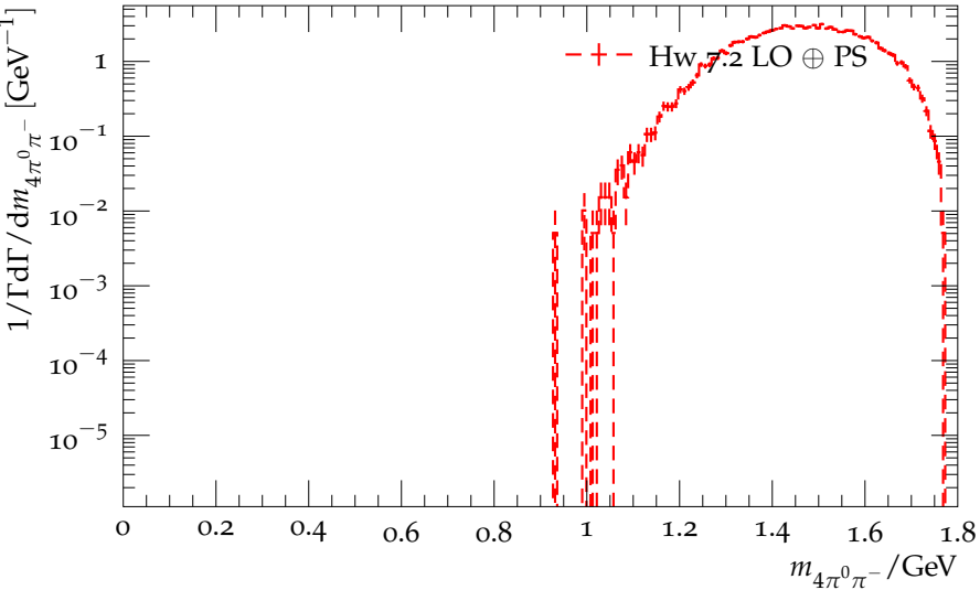
Mass distribution of the hadrons for \tau^- \rightarrow 4\pi^0 \pi^- \nu_\tau
