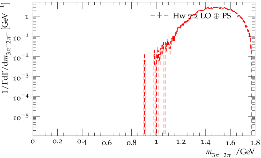
Mass distribution of the hadrons for \tau^- \rightarrow 3\pi^- 2\pi^+ \nu_\tau
