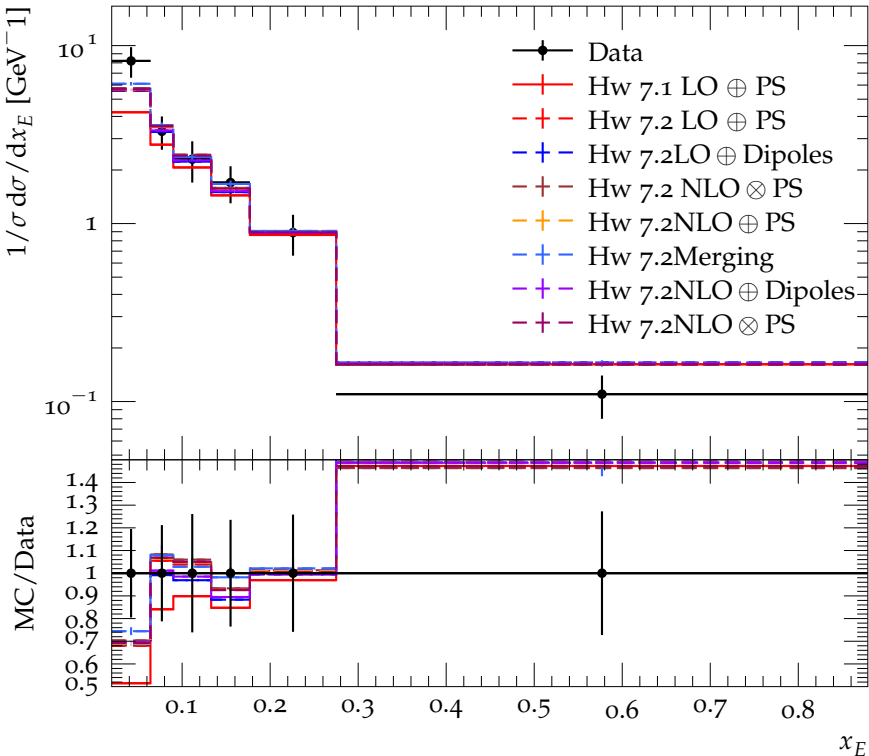
K^{*\pm} (892) cross section as function of x_E
