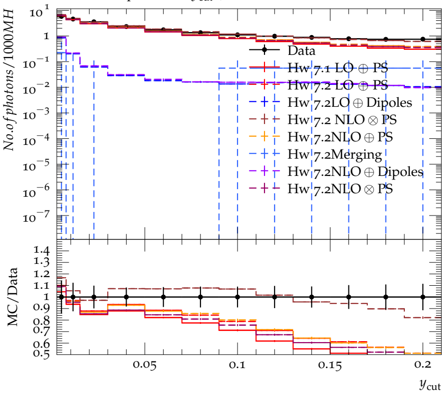
Number of photon vs y_{cut} , Jade
