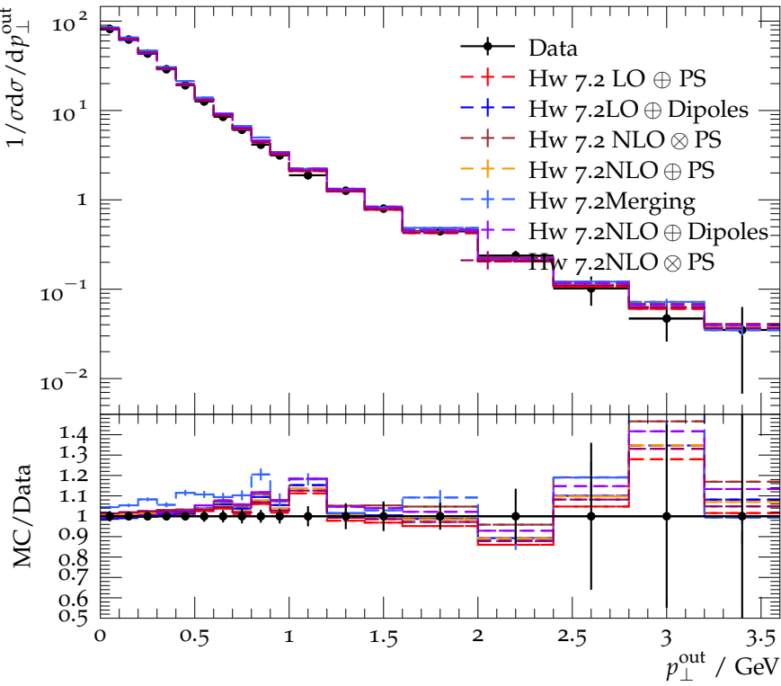
Out-of-plane p_{\perp} in GeV w.r.t. thrust axes
