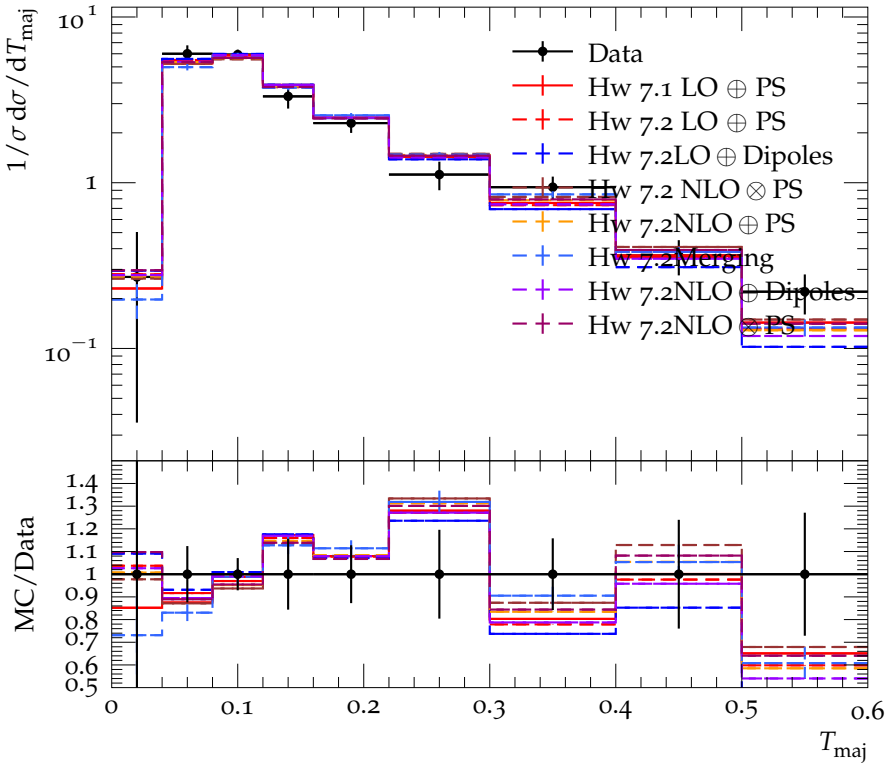
Thrust major, T_{\text{maj}} , at 133 GeV
