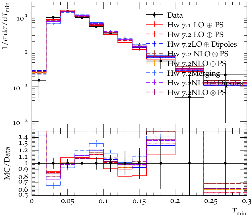
Thrust minor, T_{\min} , at 177 (161–183) GeV
