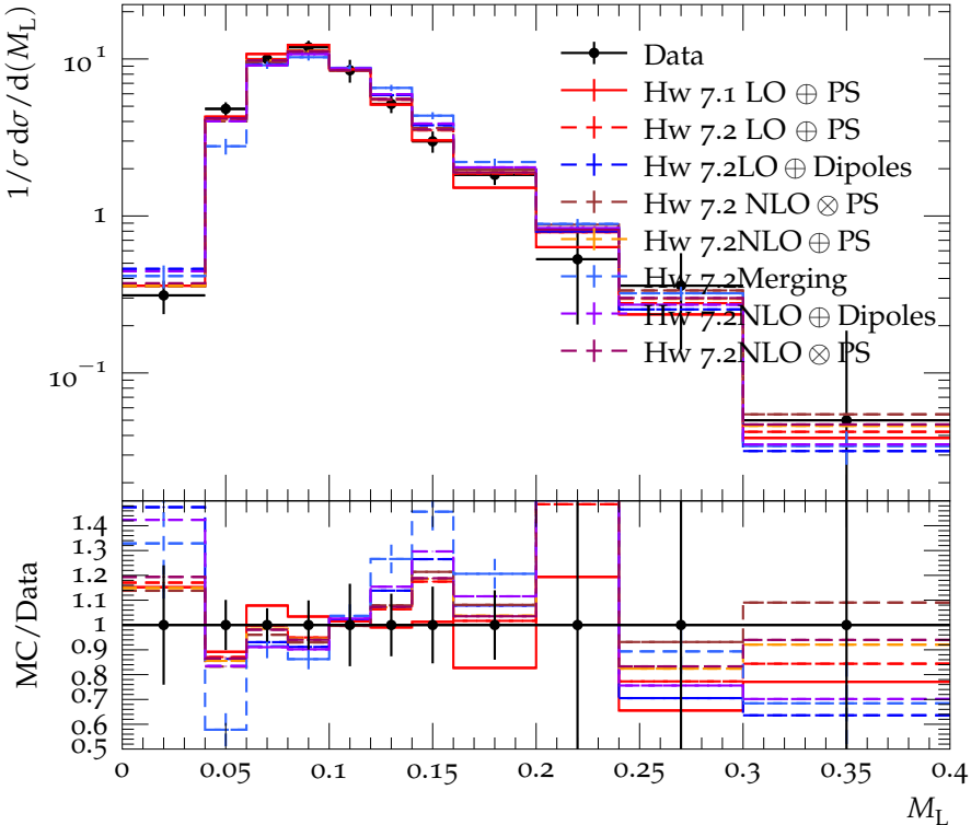
Light hemisphere mass, M_L , at 177 (161–183) GeV
