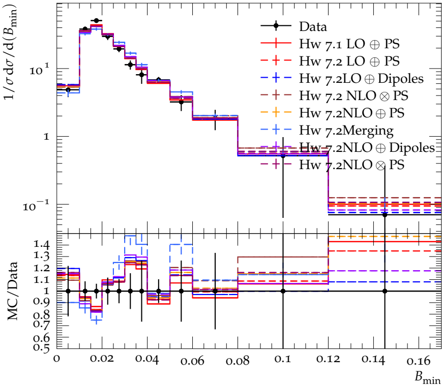
Narrow hemisphere broadening, B_{\min} , at 177 (161–183) GeV
