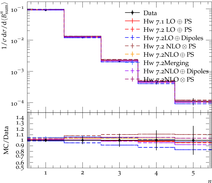
Moments of B_{\text{sum}} at 177 (161–183) GeV
