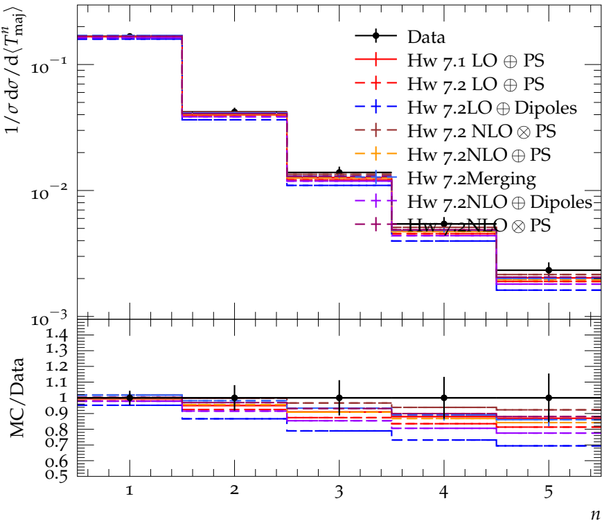
Moments of T_{\text{maj}} at 133 GeV
