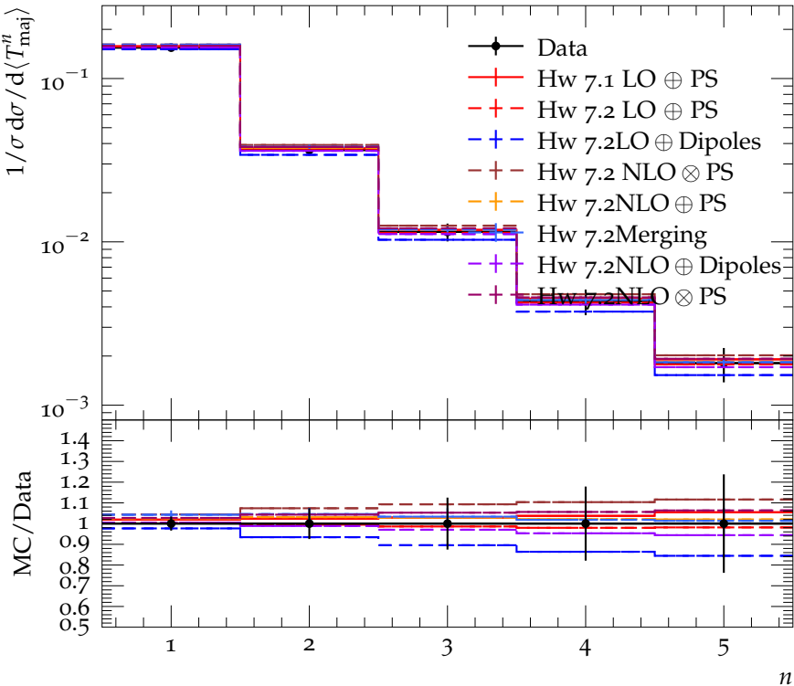
Moments of T_{\text{maj}} at 177 (161–183) GeV
