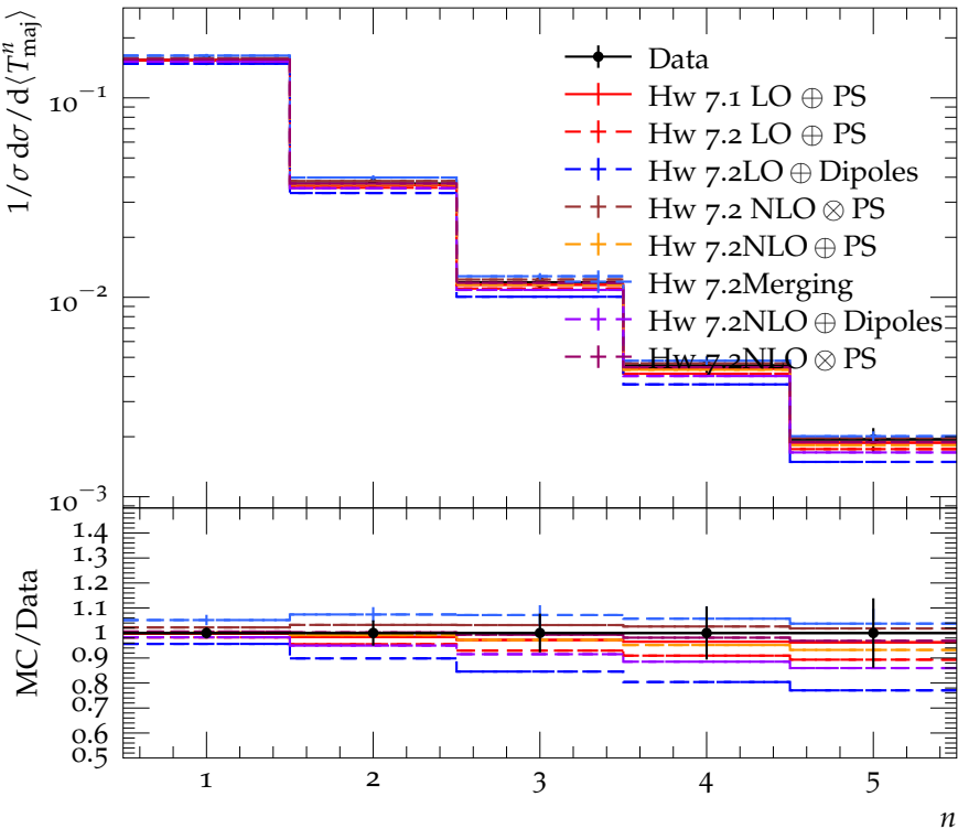
Moments of T_{\text{maj}} at 197 (189–209) GeV
