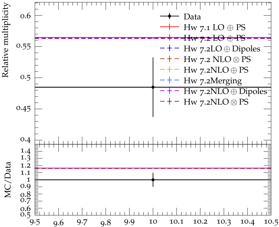
Ratio (w.r.t. \pi^\pm ) of mean \pi^0 multiplicity
