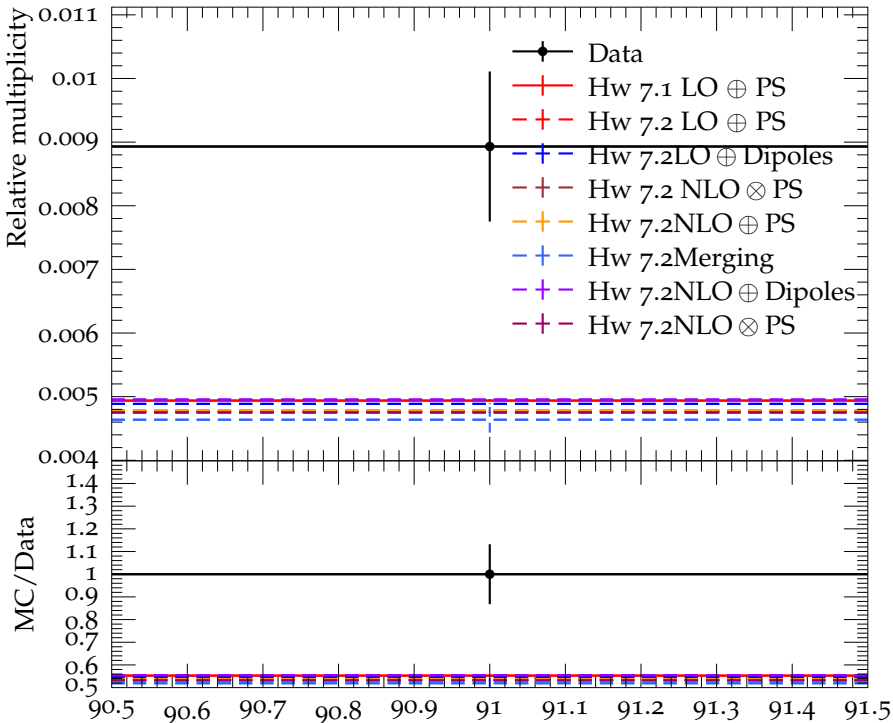
Ratio (w.r.t. \pi^\pm ) of mean \eta(\hat{958}) multiplicity
