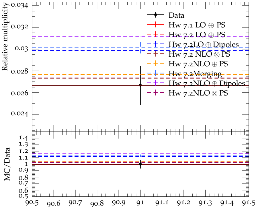
Ratio (w.r.t. \pi^\pm ) of mean D^0 multiplicity
