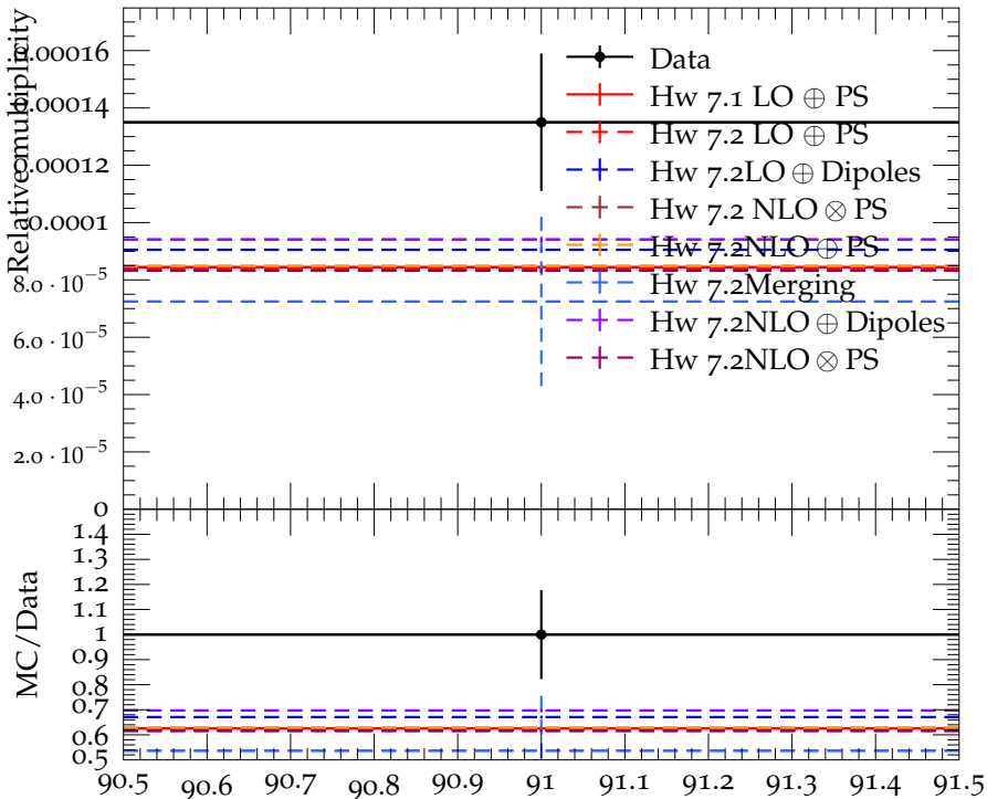
Ratio (w.r.t. \pi^\pm ) of mean \psi(2S) multiplicity
