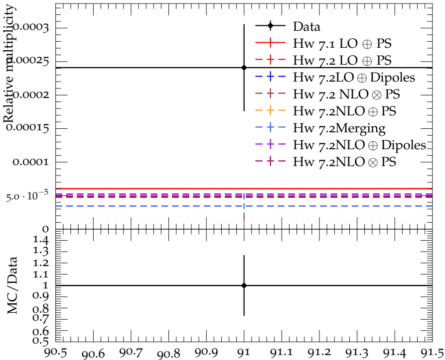
Ratio (w.r.t. \pi^\pm ) of mean \chi_{c1}(3510) multiplicity
