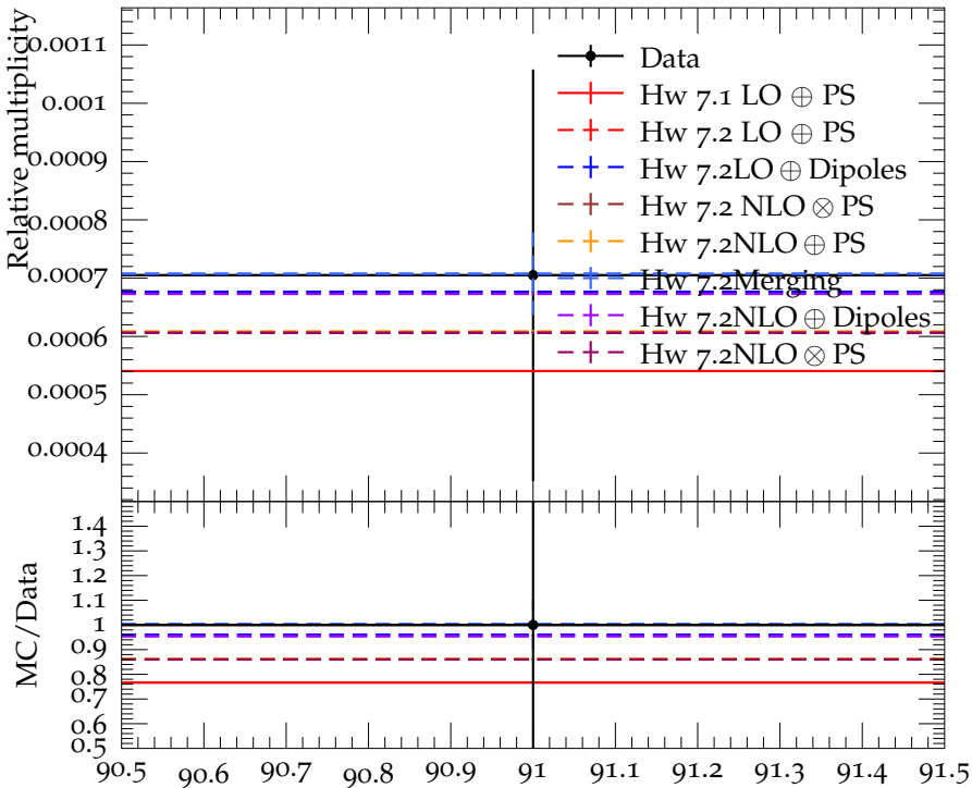
Ratio (w.r.t. \pi^\pm ) of mean f_2(1525) multiplicity
