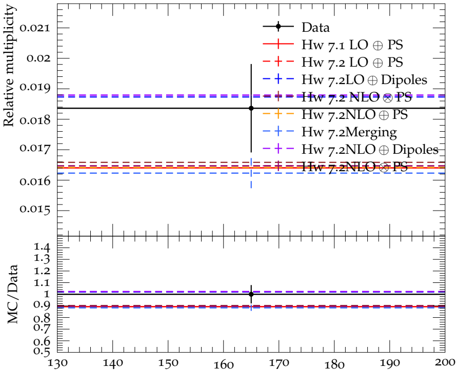
Ratio (w.r.t. \pi^\pm ) of mean \Lambda multiplicity
