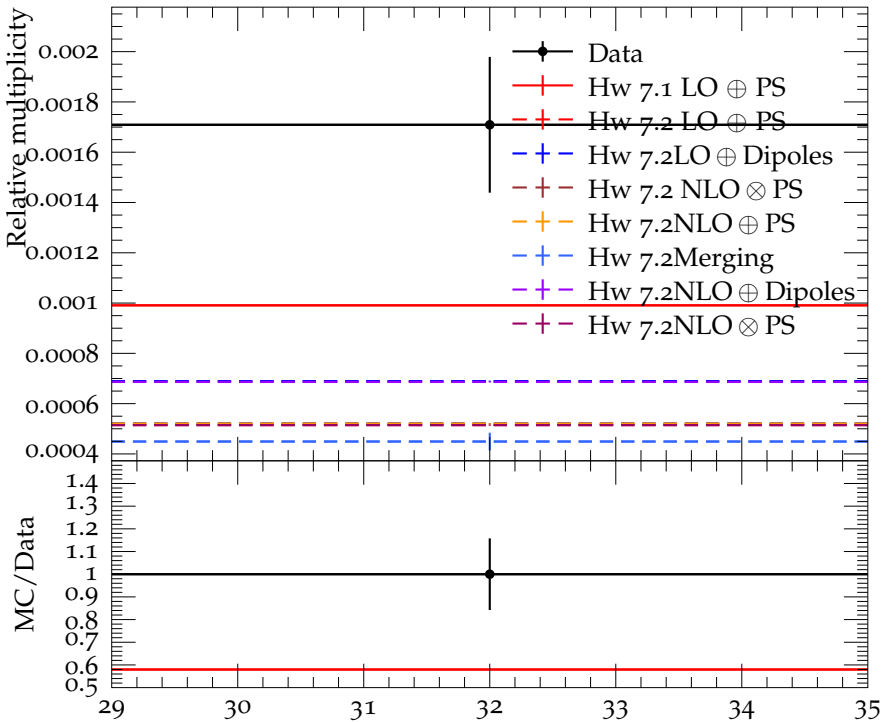
Ratio (w.r.t. \pi^\pm ) of mean \Xi^- multiplicity
