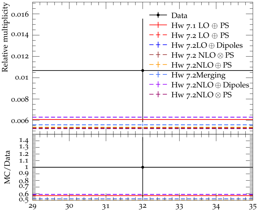
Ratio (w.r.t. \pi^\pm ) of mean \Lambda_c^+ multiplicity
