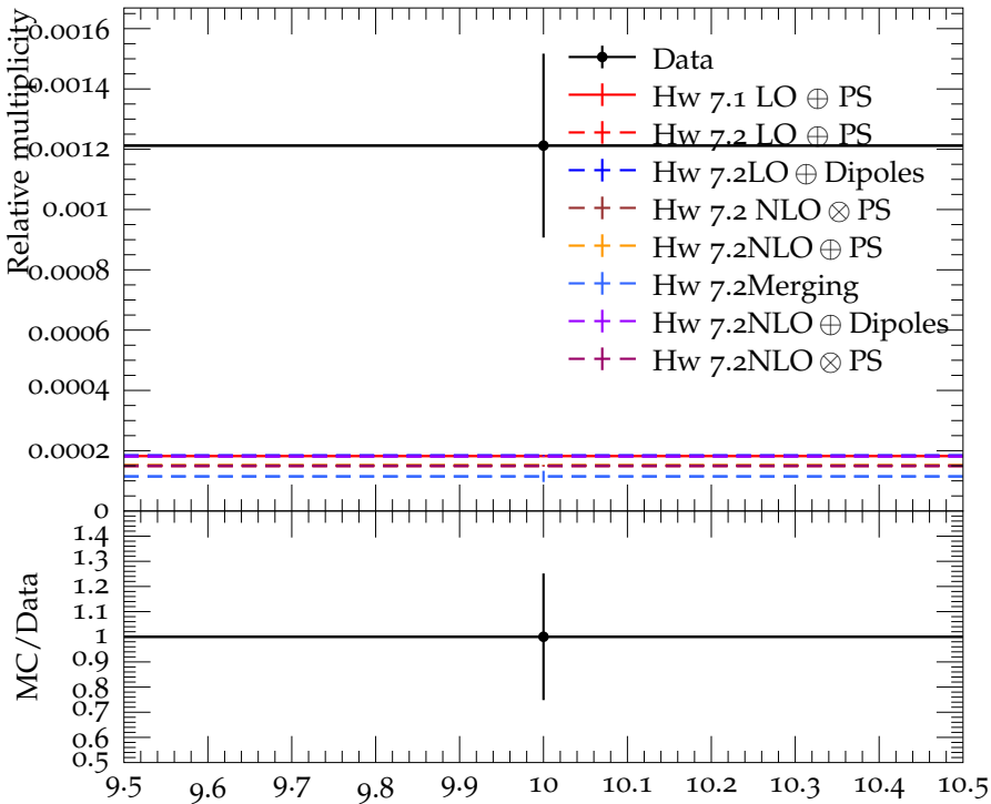
Ratio (w.r.t. \pi^\pm ) of mean \Lambda(1520) multiplicity
