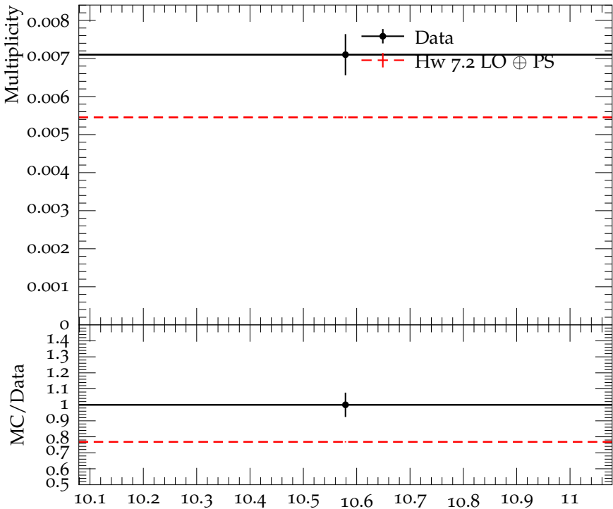
Mean \chi_{c1}(1P) multiplicity
