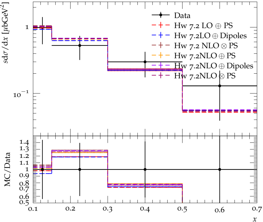
K_{S,L}^0 scaled momentum spectrum at E_{\text{CMS}} = 9.4 GeV
