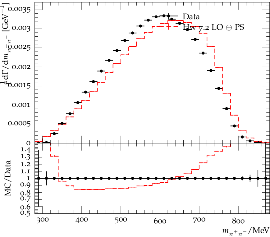
Mass distribution for \pi^+\pi^- in \phi \rightarrow \pi^+\pi^-\pi^0
