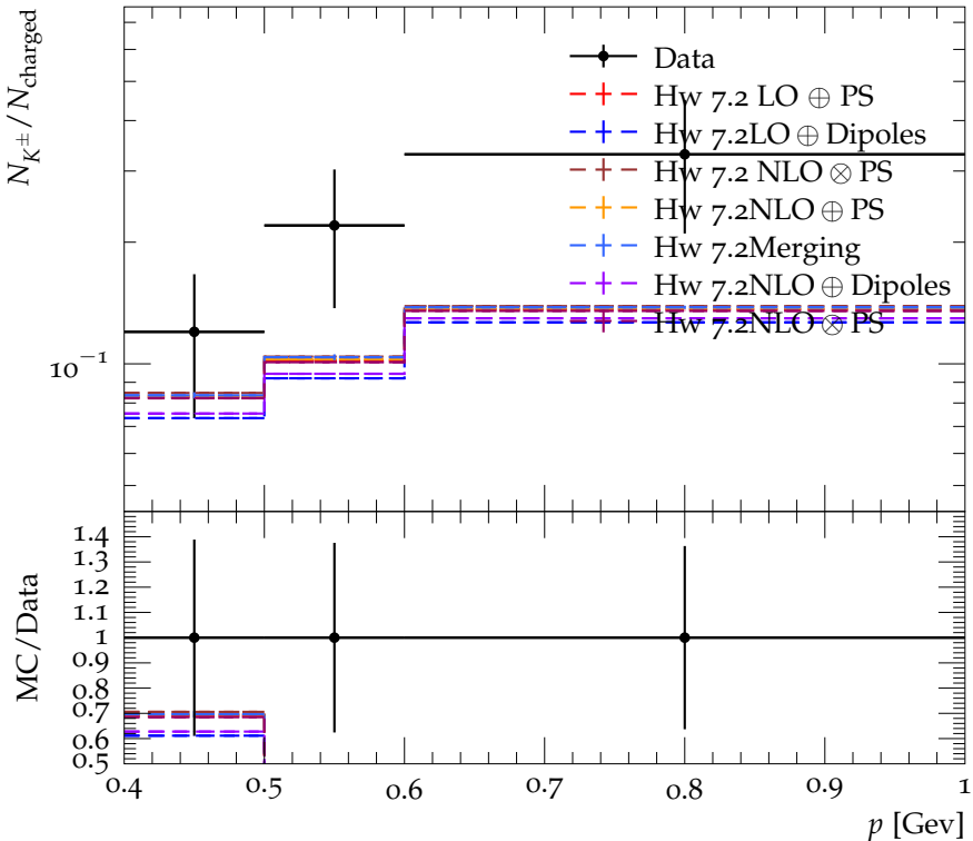
Ratio of K^\pm to charged particles at 12 GeV
