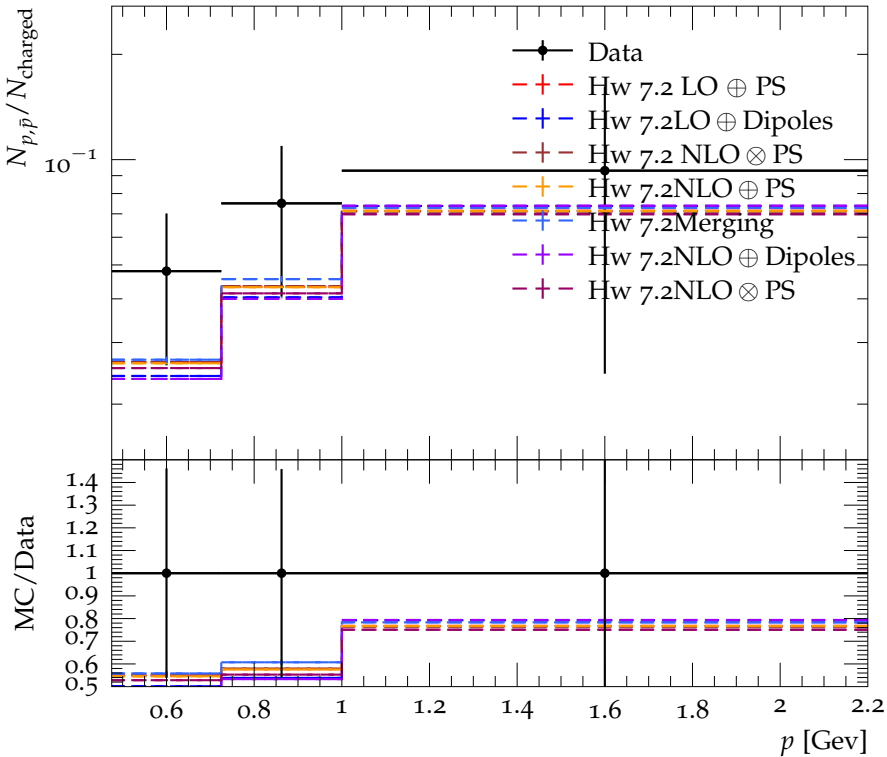
Ratio of p, \bar{p} to charged particles at 12 GeV
