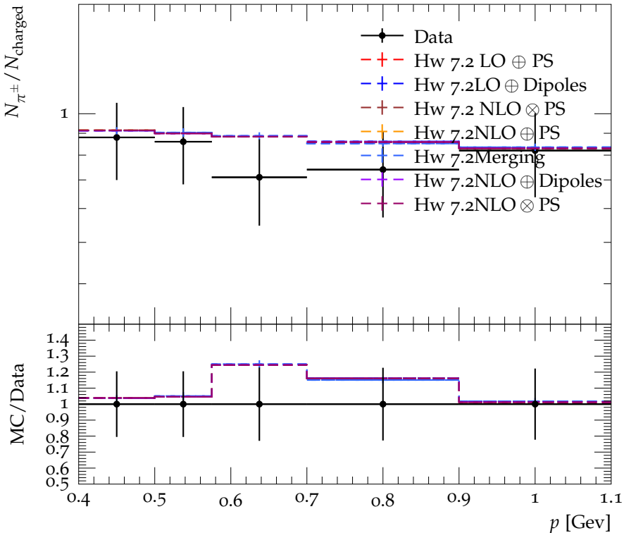
Ratio of \pi^\pm to charged particles at 30 GeV
