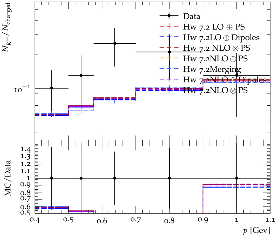
Ratio of K^\pm to charged particles at 30 GeV
