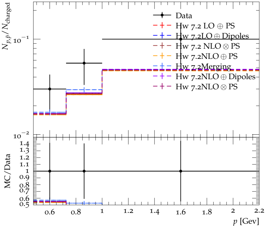
Ratio of p, \bar{p} to charged particles at 30 GeV
