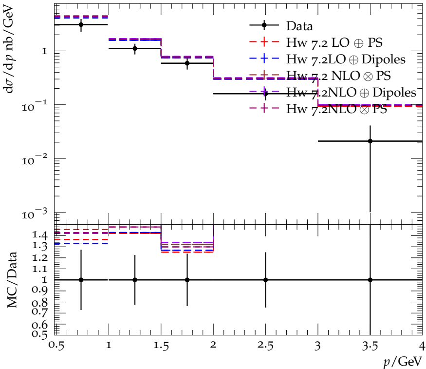
\pi^0 momentum spectrum for E_{\text{CMS}} = 14 GeV
