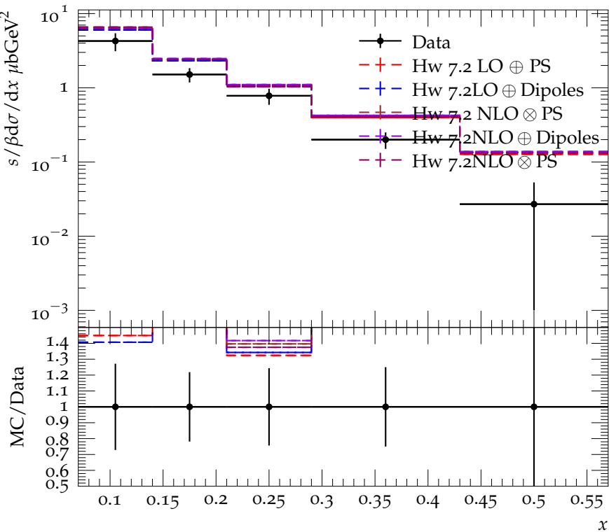
\pi^0 scaled momentum spectrum for E_{\text{CMS}} = 14 GeV
