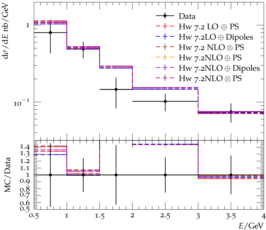
\pi^0 energy spectrum for E_{\text{CMS}} = 34 GeV
