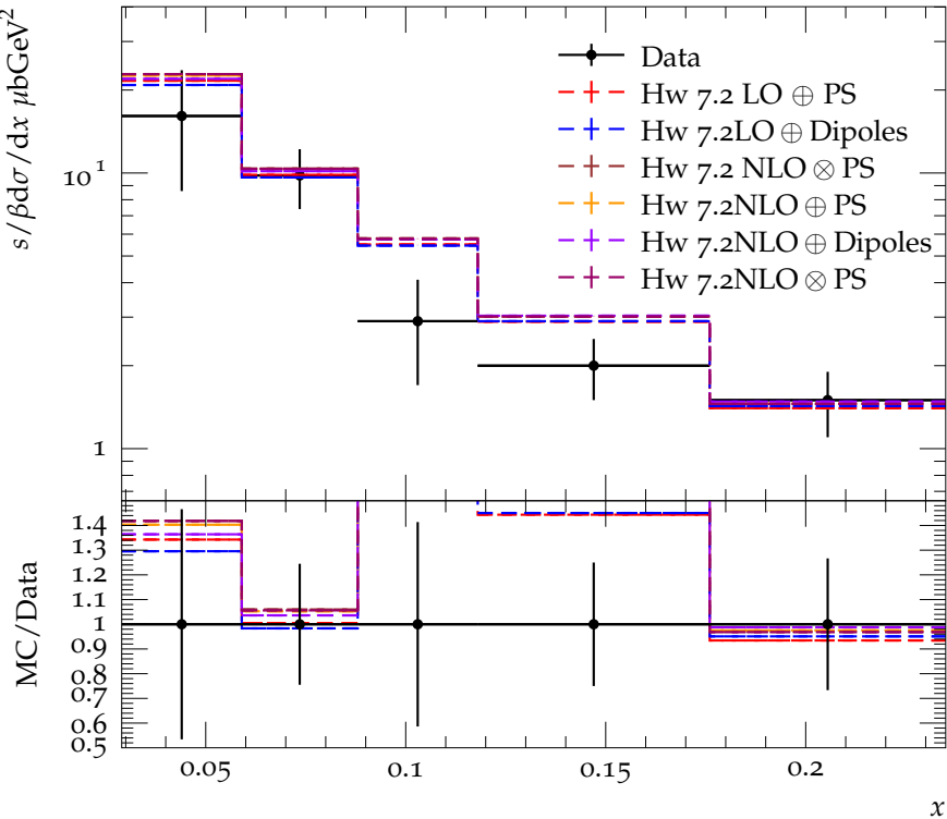
\pi^0 scaled momentum spectrum for E_{\text{CMS}} = 34 GeV
